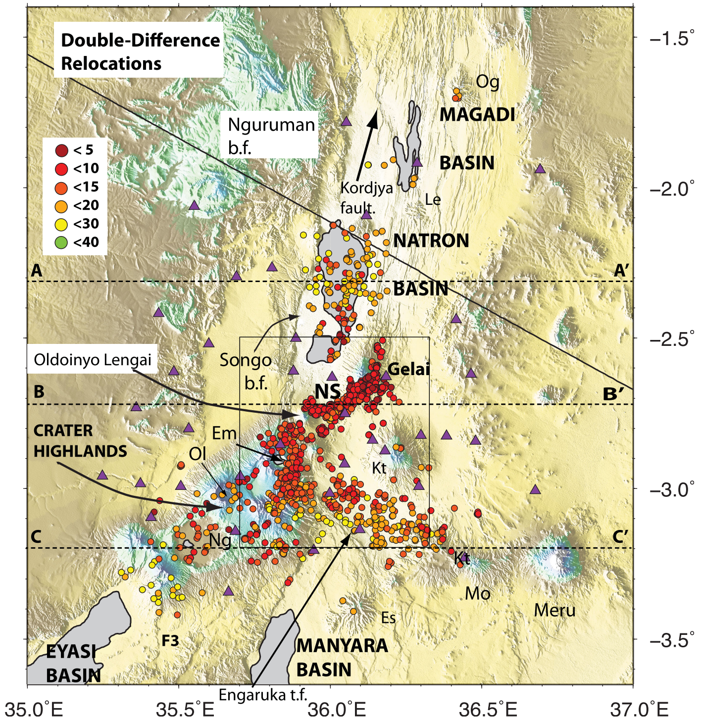
Figure 6. Earthquake locations from the double-difference analyses of catalogue times and P wave cross correlations, combined from smaller bins spanning the network. See text for details of catalogue and cross-correlation weightings. Epicenters are color coded by depth. Labels refer to volcanoes NS = Naibor Soito monogenetic cone field; Em = Embagai; Ol = Olmoti; Kt = Kitumbeine; Ng = Ngorongoro; Es = Essimngor; Mo = Monduli. F3 is an unnamed normal fault. Cross sections in Figure 9 are E-W profiles at 2.3°S (A–A’), 2.72°S (B–B’), and 3.2°S (C–C’). Epicentral locations in 10 km-wide swath centered on each line are projected onto the line of each cross section.
