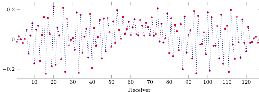
Figure 9: Real part of hard-diffracted wave at 128 receptors for FSSL 4 \cdots\cdots and MJ Q8 Raf \circ . Rel L^2 error is 1.48 \times 10^{-4} . ( Num. Exp. 3 )
