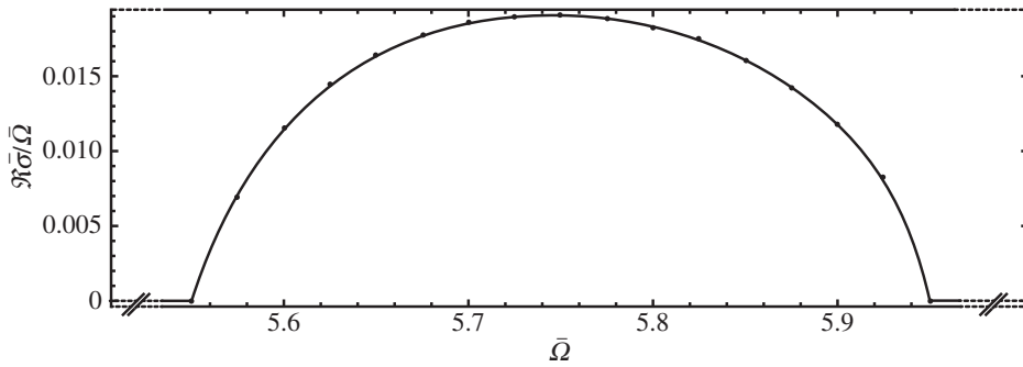
Figure 6. Largest growth rate \Re \bar{\sigma} predicted by the linear stability analysis described in appendix B, as a function of the angular velocity \bar{\Omega} . The same parameter values are used as in the experiments (S3c), namely \bar{R} = 0.032 and \bar{L}_s = 0.29 . An instability is present in a small range of values of \bar{\Omega} around \bar{\Omega} = 5.75 . There, the maximum growth rate remains small \Re \bar{\sigma} = 0.019\bar{\Omega} . A more detailed investigation of the range of unstable parameters is presented in figure 8.
