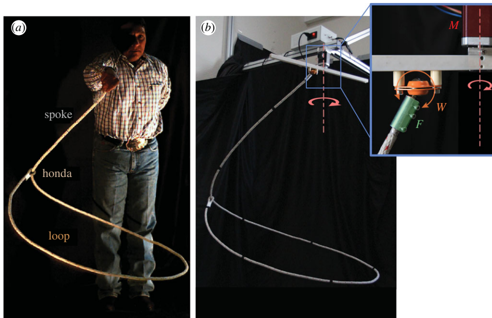
Figure 2. (a) A trick roping expert (Jesus Garcilazo (JG)) performing the Flat Loop trick. The lasso has a (total) curvilinear length L and comprises a spoke of length L_s and a loop of length L_l = L - L_s , connected by a slipknot (the honda). (b) The experimental set-up ('robo-cowboy'). The upper end of the rope is fixed in a cylindrical metal housing ( F ) that is free to rotate about its axis, and which is analogous to the trick roper's fingers. The upper end of the housing is in turn attached to a pivot ( W ) that is analogous to the roper's wrist. Finally, the pivot is attached to a bar that is rotated in a horizontal plane by a motor M . (Online version in colour.)
