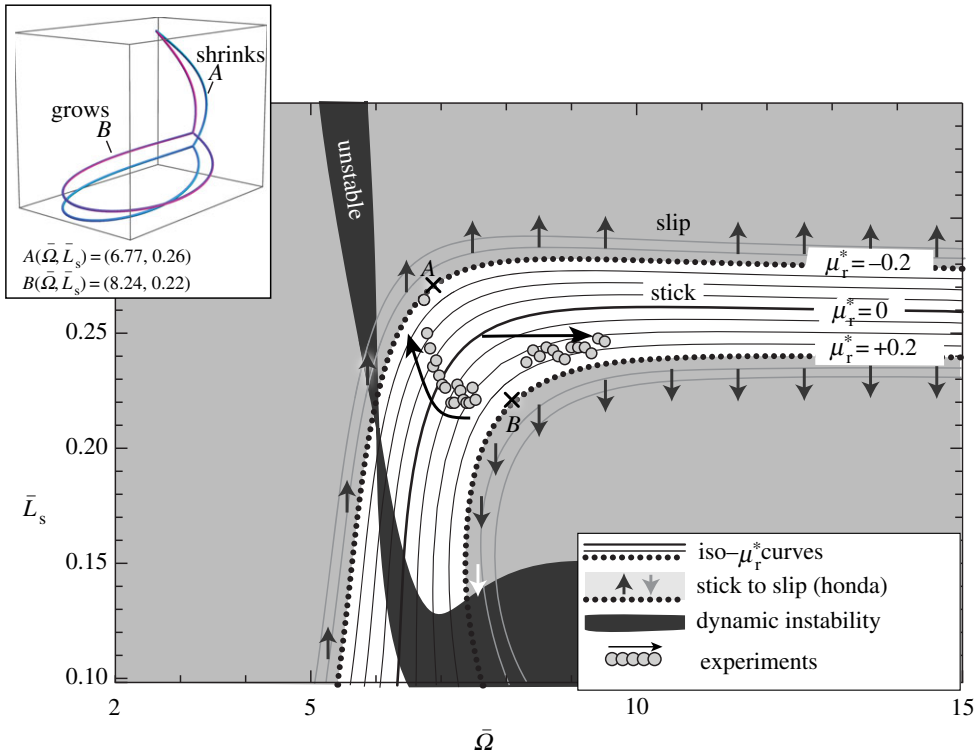
Figure 8. Diagram of stability of the lasso in the (\bar{\Omega}, \bar{L}_s) plane, for \bar{R} = 0.032 . The parallel black and grey curves show the isovalues of \mu_r^* predicted by the matched asymptotic expansions: the central thick black curve corresponds to frictionless solutions ( \mu_r^* = 0 ), and the black dotted curves show the onset of sliding ( \mu_r^* = \pm\mu_r ) at the honda for a Coulomb coefficient \mu_r = 0.2 . Two particular configurations on these curves are shown in insets A and B . Near the dotted curves, the grey (unstable) and white (stable) arrows represent the lasso behaviour after the onset of sliding at the honda, as discussed in the main text. The dark grey region marks the linearly unstable domain based on the stability analysis of appendix B. Grey dots correspond to two experimental datasets ( R = 12.7 cm, L = 396 cm, corresponding to the same \bar{R} = 0.032 ), obtained with a cotton lasso for slowly increasing and decreasing angular frequencies; the arrows indicate the order in which these points were measured. (Online version in colour.)
