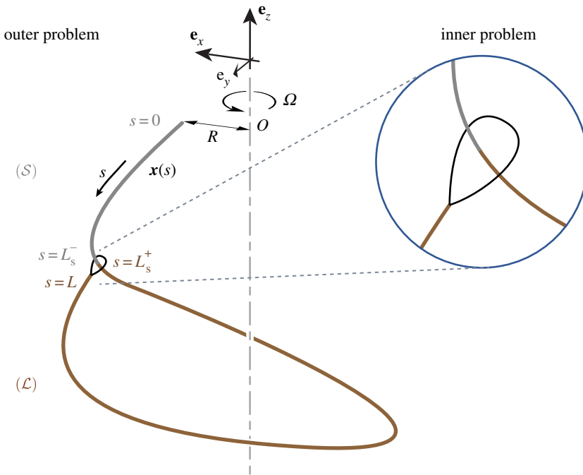
Figure 3. The Flat Loop trick is described mathematically as static solutions in a rotating frame of an inextensible string or elastic rod held at a distance R from the axis. (Online version in colour.)
