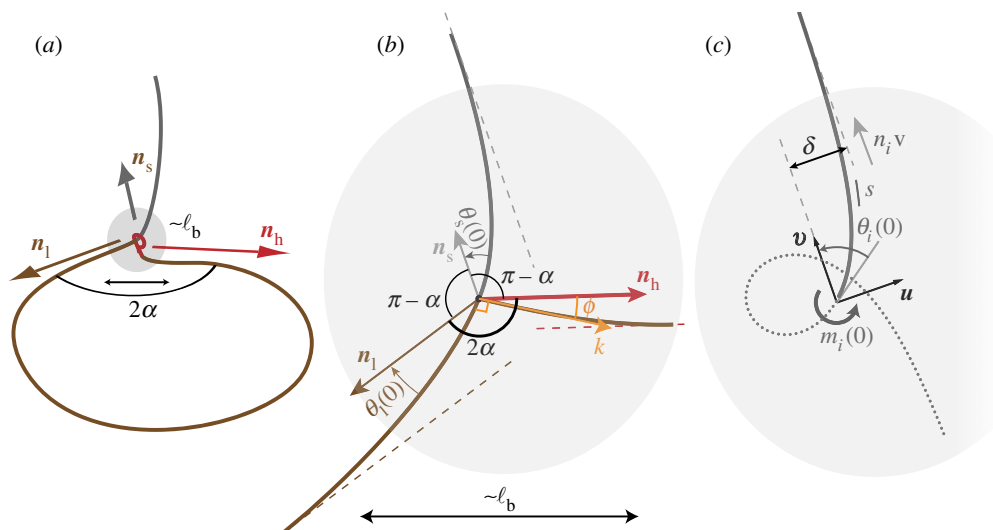
Figure 7. (a) Sketch of the global solution: the outer (string) solution is valid far from the honda and has to be matched with the inner solution inside the shaded disc. The equilibrium of the honda, \mathbf{n}_s + \mathbf{n}_l + \mathbf{n}_h = \mathbf{0} , implies that the inner problem is planar. By the analysis of the outer (string) problem, we know that the loop is symmetric and define \alpha to be half its angle at the honda. (b) The inner problem, of typical size \ell_b . (c) Elastica solution relevant to either of the strands s or l . (Online version in colour.)
