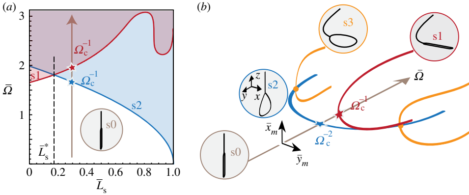
Figure 9. Bifurcation analysis of a lasso with a non-sliding honda ( \mu_r = \infty ), with the upper endpoint lying on the axis ( \bar{R} = 0 ). Flat Loops are obtained from the unbuckled (straight, vertical) configuration s_0 by a succession of two bifurcations. (a) Bifurcation analysis of the unbuckled configuration s_0 showing a competition of the whirling instability ( s_1 : loop stays closed, string becomes curved) and ‘coat-hanger’ instability ( s_2 : loop opens up, spoke remains straight): the critical rotation frequencies are plotted as a function of the spoke length \bar{L}_s . The coat-hanger mode occurs first when \bar{L} > \bar{L}_s^* = 0.167 . (b) Bifurcation diagram as a function of the rotation frequency \bar{\Omega} , for \bar{L}_s = 0.29 , showing the branches corresponding to the trivial solution ( s_0 ), the whirling modes ( s_1 ), the hanger mode ( s_2 ) and the Flat Loop mode ( s_3 ). The unbuckled solution first becomes unstable to a hanger mode (planar solution with open loop, s_2 ); at a higher frequency, the hanger mode loses planar symmetry and goes to a lasso shape, s_3 , by a secondary bifurcation. (Online version in colour.)
