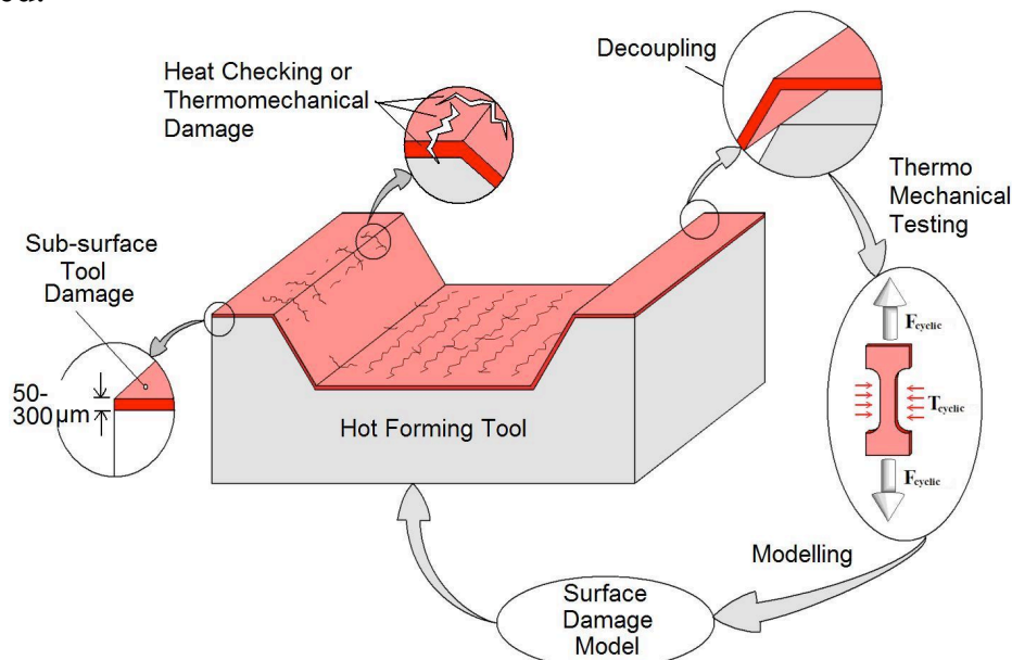
Figure 1. General procedure for the study of surface damage in tool steels.
