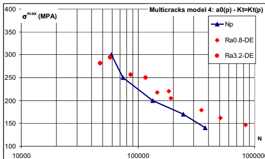
Fig. 15. Fatigue life prediction given with model 4.
