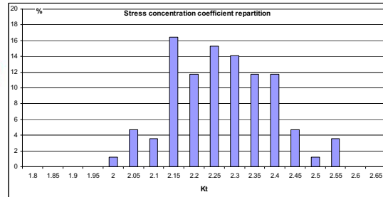
Fig. 11. Statistical distribution of stress concentration coefficient.
