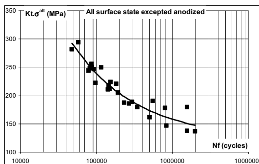
Fig. 8. Fatigue results using K_{t_{local}} method for all surface treatments excepted anodizing and for the two initial surface roughness.
