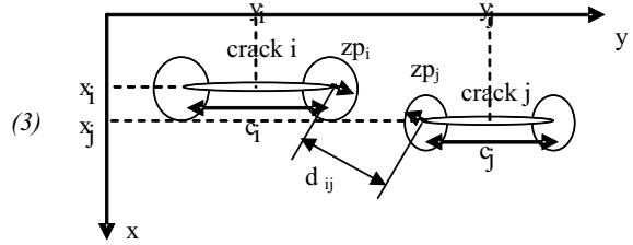
Fig. 5. Coalescence criteria conventions.
