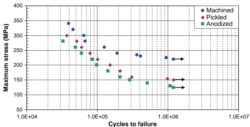
Fig. 8. Fatigue test results for as machined, pickled and anodized specimens.
