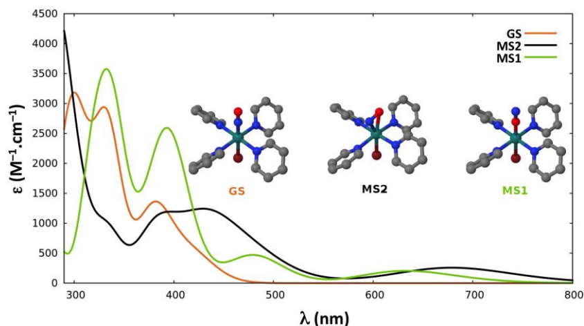
Figure 4. TD-DFT absorption spectra of the three linkage isomers ( GS in orange, MS2 in black, and MS1 in green) of trans\text{-}[\text{RuBr}(\text{NO})(\text{py})_4]^{2+} . Broadening model used: Gaussian function with a half-width at half-height of 0.2 eV.
