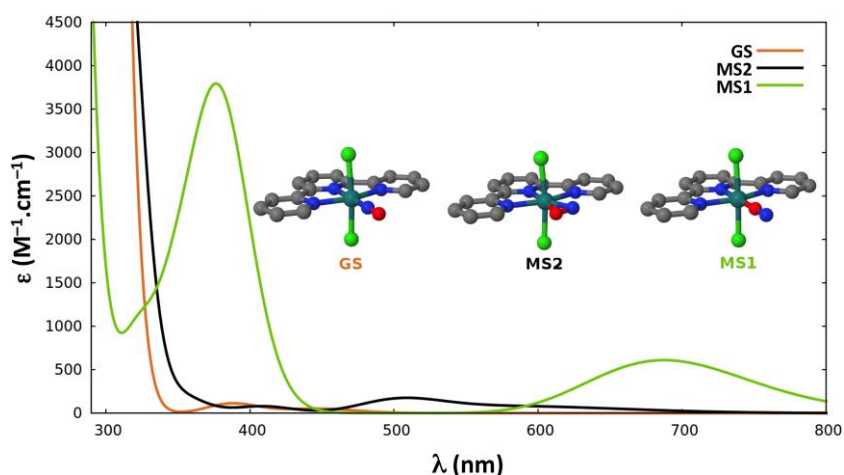
Figure 5. TD-DFT absorption spectra of the three linkage isomers ( GS in orange, MS2 in black, and MS1 in green) of trans\text{-}(\text{Cl},\text{Cl})[\text{RuCl}_2(\text{NO})(\text{tpy})]^+ . Broadening model used: Gaussian function with a half-width at half-height of 0.2 eV.
