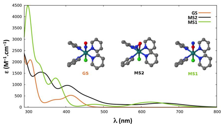
Figure 3. Time-dependent DFT (TD-DFT) absorption spectra of the three linkage isomers (GS in orange, MS2 in black, and MS1 in green) of trans -[RuCl(NO)(py) 4 ] 2+ . Broadening model used: Gaussian function with a half-width at half-height of 0.2 eV.
