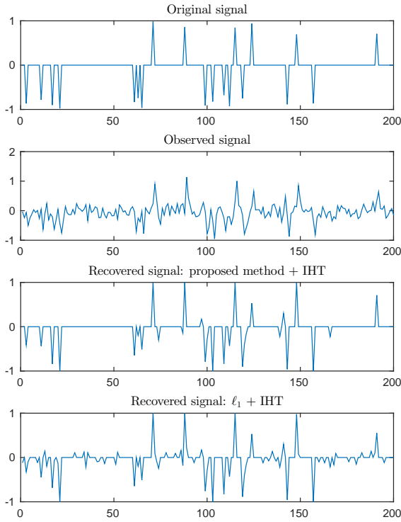
Fig. 2. Typical original signal \bar{\mathbf{x}} , observations \mathbf{y} and recovered signal. The results presented have been obtained with IHT initialized either by our method or by a linearized model and \ell_1 penalty.
