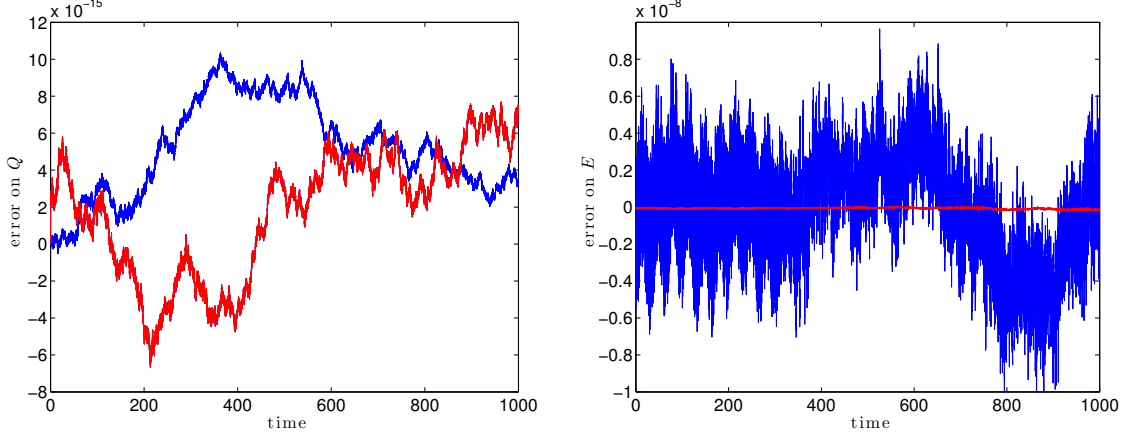
(a) quadratic invariant error.
