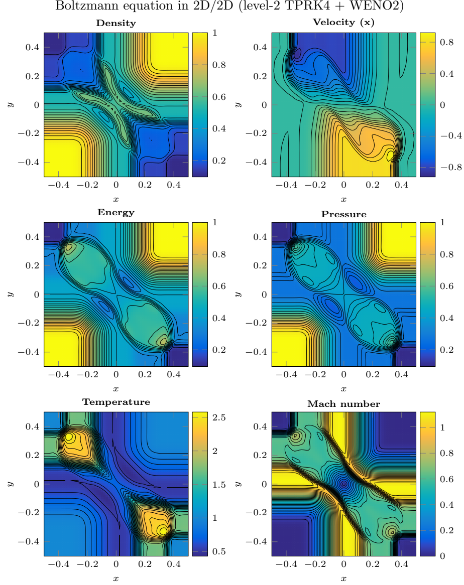
Figure 12: Numerical solution of the Boltzmann equation with pseudo-Maxwellian particles in 2D/2D at t = 0.16 for a double Sod shock test (51). Velocity space is discretized using J_x = J_y = 32 . We applied a level-2 TPRK4 method with FE as innermost integrator and h_0 = \varepsilon = 5 \cdot 10^{-5} together with WENO2 with I_x = I_y = 64 .
