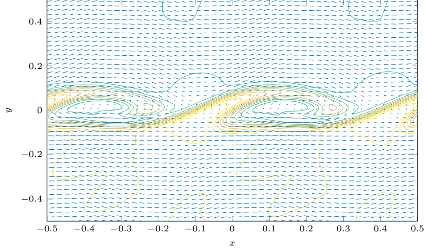
Figure 11: Velocity field and density line of the Kelvin-Helmoltzm-like instability at time t = 0.9 .
