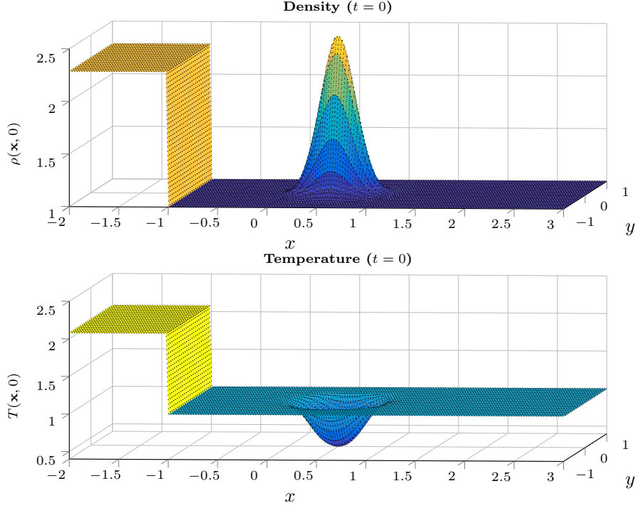
Figure 7: Initial solution for density (top) and temperature (bottom) of the shock-bubble interaction in 2D/2D. The spatial domain [-2, 3] \times [-1, 1] is discretized using I_x = 200 and I_y = 25 .
