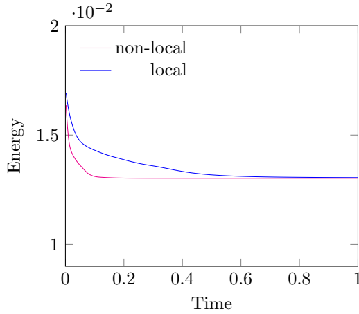
FIGURE 1. Evolution of the energy \mathcal{E}(\mathbf{c}) along time for the non-local model (17) and the local one (22). The decay of the energy is faster for the non-local model, as shown in Section 1.3.
