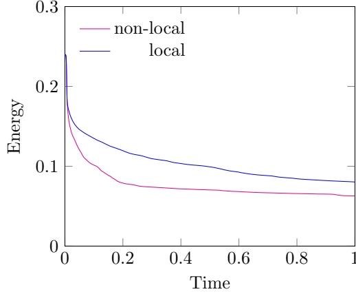
FIGURE 4. Evolution of the energy \mathcal{E}(\mathbf{c}) along time for the non-local model (17) and the local one (22) for the spinodal decomposition test case.
