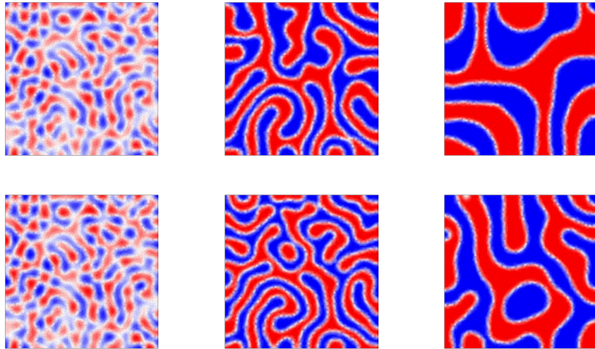
FIGURE 3. Snapshots at times t = 6 \cdot 10^{-3} (left), t = 5 \cdot 10^{-2} (middle), and t = 1 (right) illustrating the spinodal decomposition governed by model (17) (top) and model (22) (bottom).
