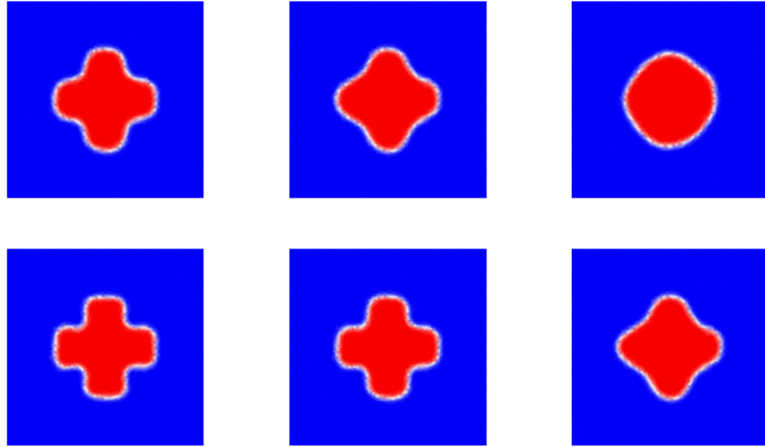
FIGURE 2. Evolution along time of the numerical solution to the non-local problem (17) (top) and to the local problem (22) (bottom). Snapshots at time t = 10^{-2} (left), t = 2 \cdot 10^{-2} (middle), and t = 10^{-1} (right).
