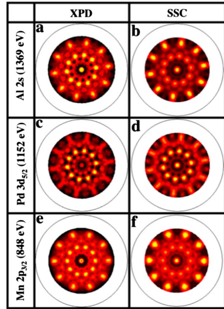
FIG. 9. (Color online) Experimental XPD patterns of (a) Al 2s , (c) Pd 3d_{5/2} , and (e) Mn 2p_{3/2} core levels measured on the T- \text{Al}_3(\text{Mn,Pd}) (010) surface with Al K\alpha (1486.7 eV) x-ray source. Single scattering cluster simulations for (b) Al 2s ( E_{Kin}=1369 eV), (d) Pd 3d_{5/2} ( E_{Kin}=1152 eV), and (f) Mn 2p_{3/2} ( E_{Kin}=848 eV) emissions based on a cluster derived from the bulk model (Ref. 17) described in Fig. 1.
