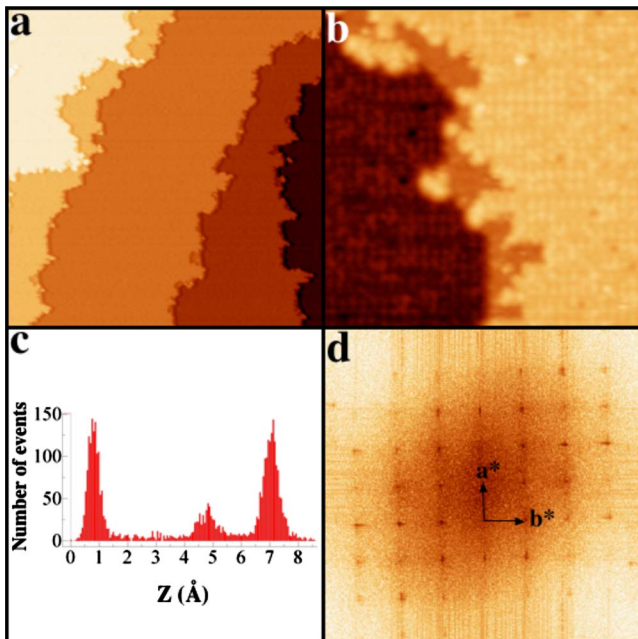
FIG. 3. (Color online) (a) STM image ( 250\times 250 nm 2 ) showing the step and terrace morphology. (b) STM image ( 40\times 40 nm 2 ) showing a narrow terrace on the step edge. (c) The height histogram calculated from a 20\times 20 nm 2 STM image exhibits the three possible step heights observed across terraces. (d) Fast Fourier transform calculated from a 50\times 50 nm 2 high-resolution STM image.
