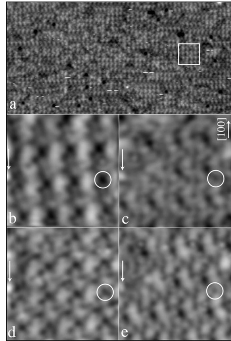
FIG. 4. (a) 70\times 35 nm 2 STM image recorded on a terrace for V_b=2 V and I_t=0.06 nA. The white frame outlines a patch of homogeneous contrast. [(b)–(e)] STM images ( 5.1\times 5.1 nm 2 ) acquired on the same region using a constant current of 40 pA and a bias of (b) 0.8 V, (c) -0.8 V, (d) 0.4 V, and (e) -0.4 V. The arrows point to a common defect visible on all images. As shown by the circles located at the same position on all images, the contrast varies drastically with the applied bias.
