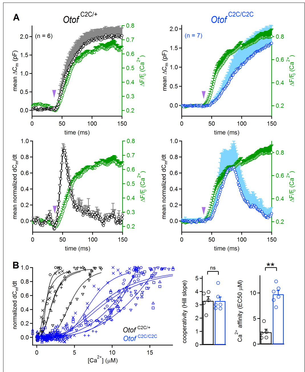
Figure 7. Reduced \text{Ca}^{2+} -sensitivity of exocytosis in Otof C2C/C2C IHCs. (A) Mean \Delta C_m response curves (top) and normalized exocytosis rates ( dC_m/dt ) (bottom), with mean intracellular fluorescent \text{Ca}^{2+} signals of OGB-5N (green traces) recorded simultaneously after \text{Ca}^{2+} uncaging (purple arrowhead) in P14-P16 Otof C2C/+ (in black) and Otof C2C/C2C (in blue) IHCs. (B) Left: For each recorded Otof C2C/+ (in black) and Otof C2C/C2C (in blue) IHC, the rate of exocytosis was plotted as a function of [\text{Ca}^{2+}]_i , and each data set was fitted with a Hill function y = V_{\max} \cdot x^n / (\text{EC}_{50}^n + x^n) . Right: Mean cooperativity and \text{Ca}^{2+} -affinity of release in Otof C2C/+ and Otof C2C/C2C IHCs. Note that for 3 out of 6 Otof C2C/C2C IHCs, the fit of the sigmoidal Hill function to the data was only partial. For those IHCs, the \text{Ca}^{2+} affinity was estimated as the value of [\text{Ca}^{2+}] for which dC_m/dt = 0.5 , rather than the \text{EC}_{50} of the fitted Hill function, which was larger. Data information: in (B), one IHC of each genotype was removed because of the lack of experimental points for a reliable fitting with a Hill function. In (A–B), data are presented as the mean \pm SEM. ** p < 0.01 , ns not significant (Mann-Whitney test).
