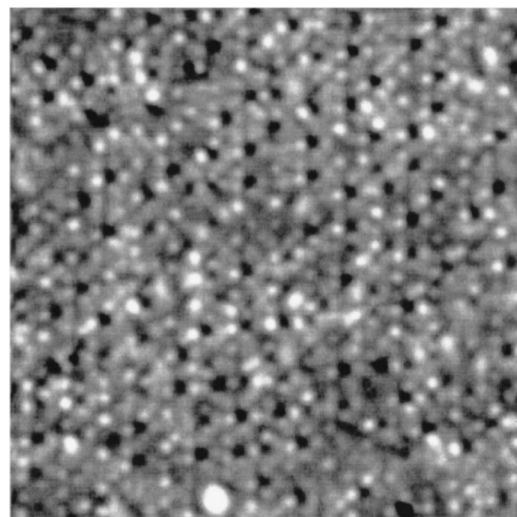
FIG. 5. High resolution STM image ( 20 \times 20 \text{ nm}^2 ) of an i\text{-Al-Pd-Mn} 5f surface, obtained under experimental conditions very similar to those of Figs. 2 and 3, and with the same experimental apparatus.
