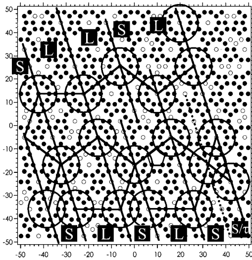
FIG. 4. Atomic positions in a plane ( 10 \times 10 \text{ nm}^2 ) generated from experimental bulk structure model. Filled circles: Al atoms. Unfilled circles: Fe atoms. The sketched contour illustrates the matching part of the STM image outlined in Fig. 3.
