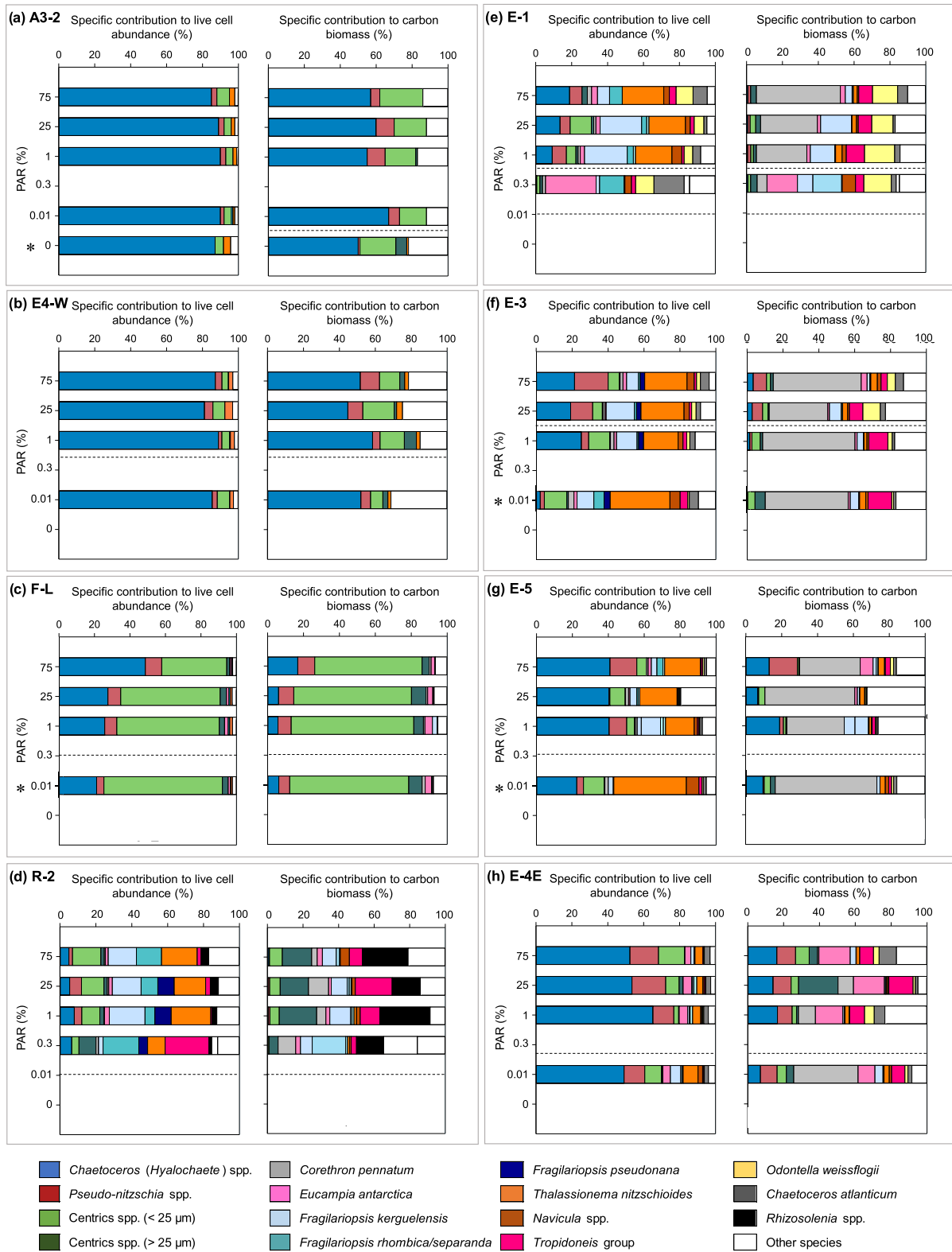
Figure 4. Vertical distributions of the relative contributions of major diatom species (as a percentage) to live cell abundance and carbon biomass at each studied station. The asterisk in front of a given light level indicates the presence of Chaetoceros resting spores. 'Other species' corresponds to low cell abundance and biomass species ( \leq 1\% of contribution). The dashed line indicates the approximate location of the mixed layer depth (MLD) and the second discontinuity observed at E-1.
