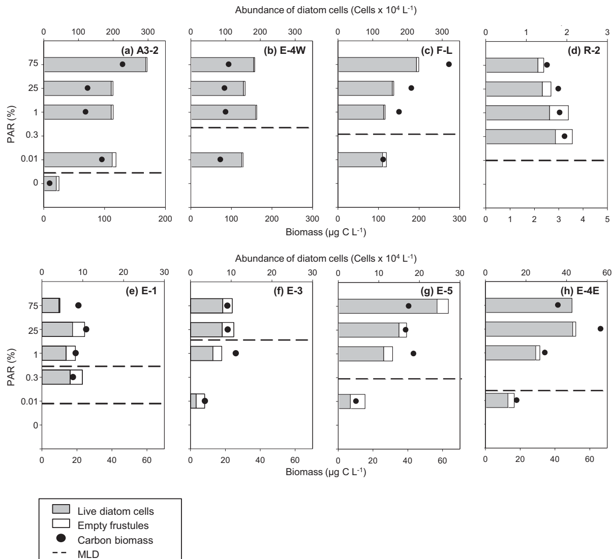
Figure 2. Vertical distributions of live cell abundance (in gray), empty frustule abundance (in white) and carbon biomass (black dots) of diatoms at each studied station. The dashed line indicates the approximate location of the mixed layer depth (MLD). A second discontinuity was identified at E-1 from the density CTD profile.
