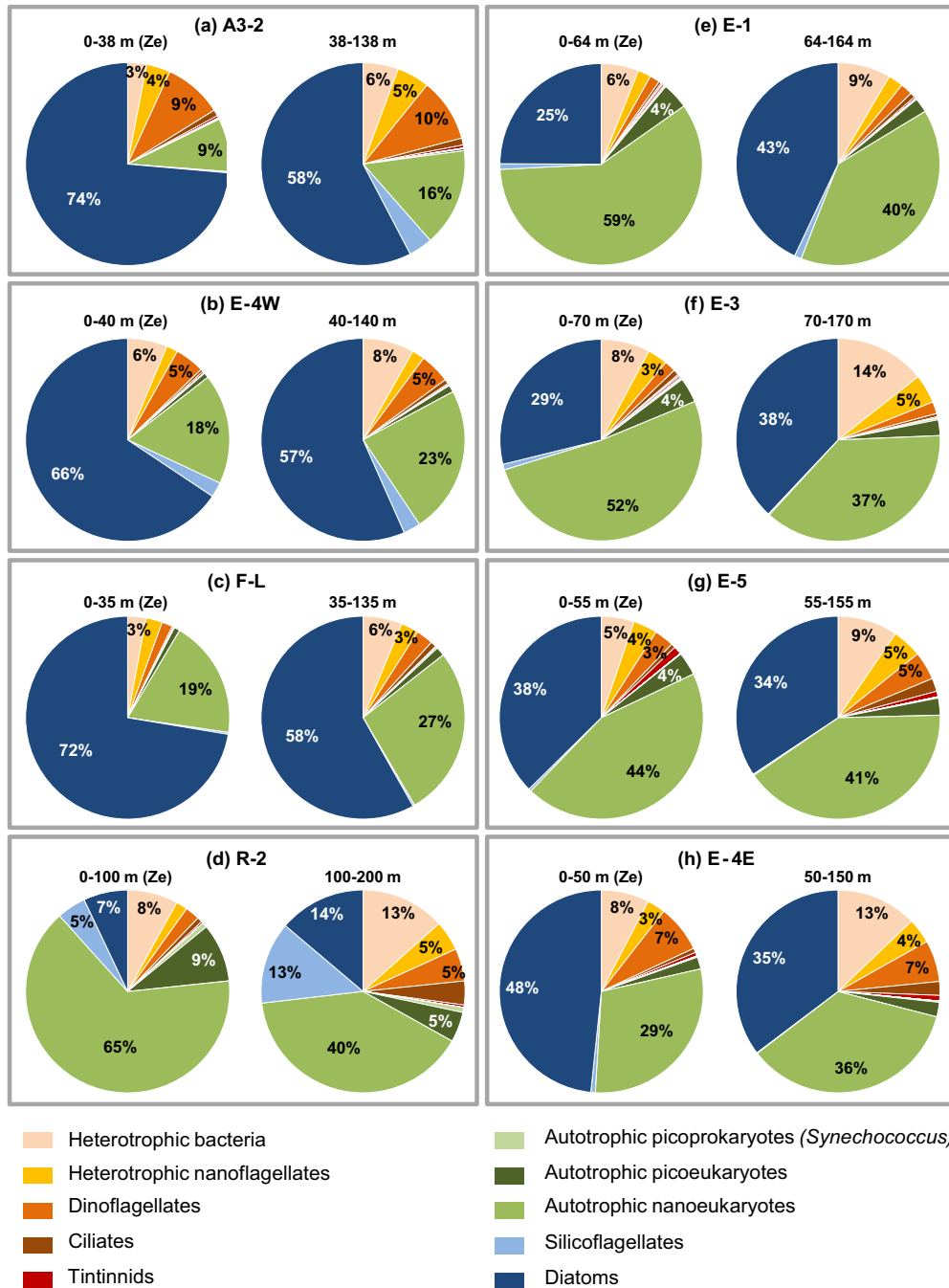
Figure 6. Relative contribution of each plankton group to carbon biomass (%) at the eight studied stations within the euphotic layer and the subeuphotic layer (defined as the layer extending 100 m below the euphotic depth, Ze). The color code ensures easy identification of autotrophic and heterotrophic organisms: blue-green colors are associated to autotrophic organisms while heterotrophic organisms are represented in red-orange.
