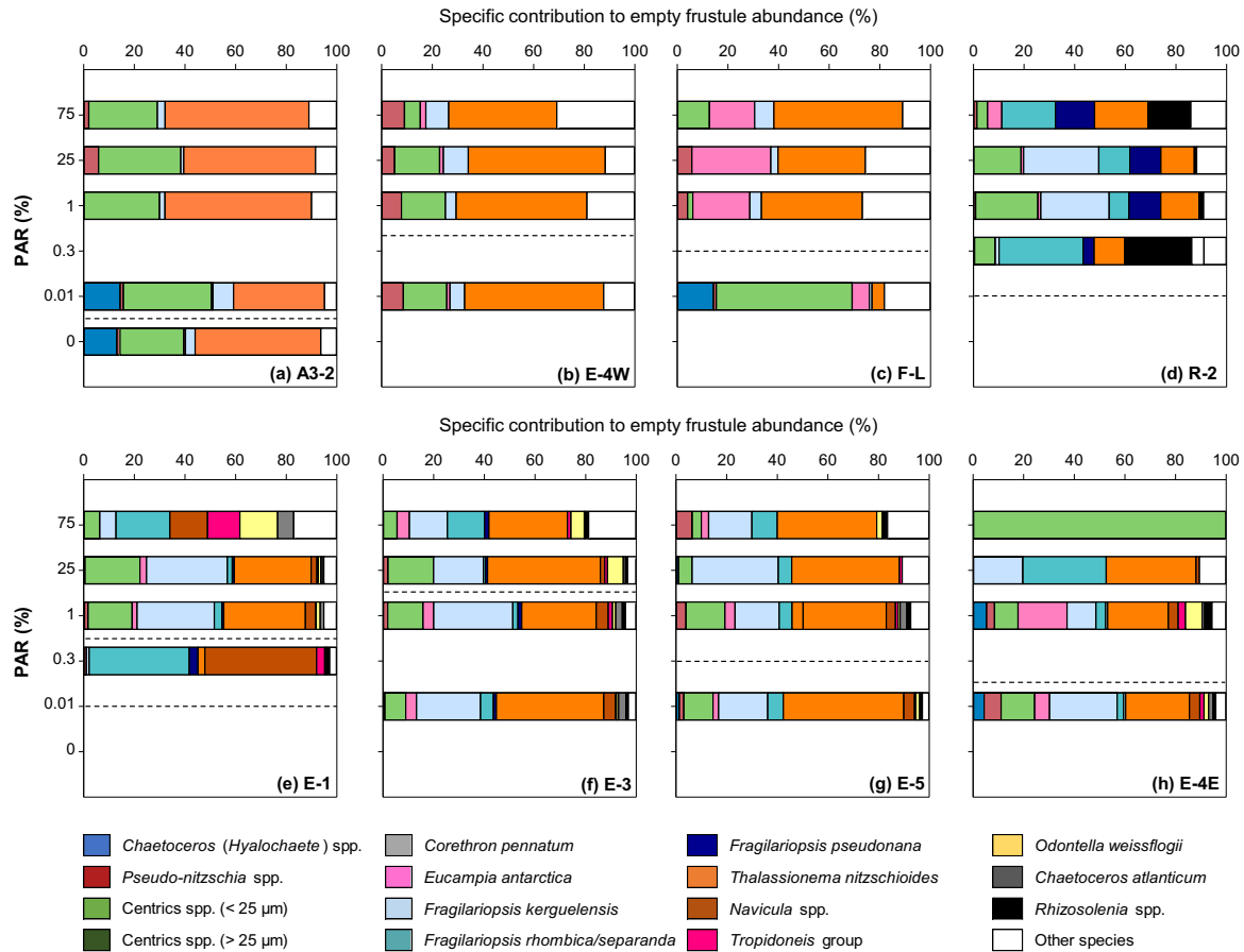
Figure 5. Vertical distributions of the relative contributions of major diatom species to empty frustule abundance (%) at each studied station. Details as in Fig. 4.
