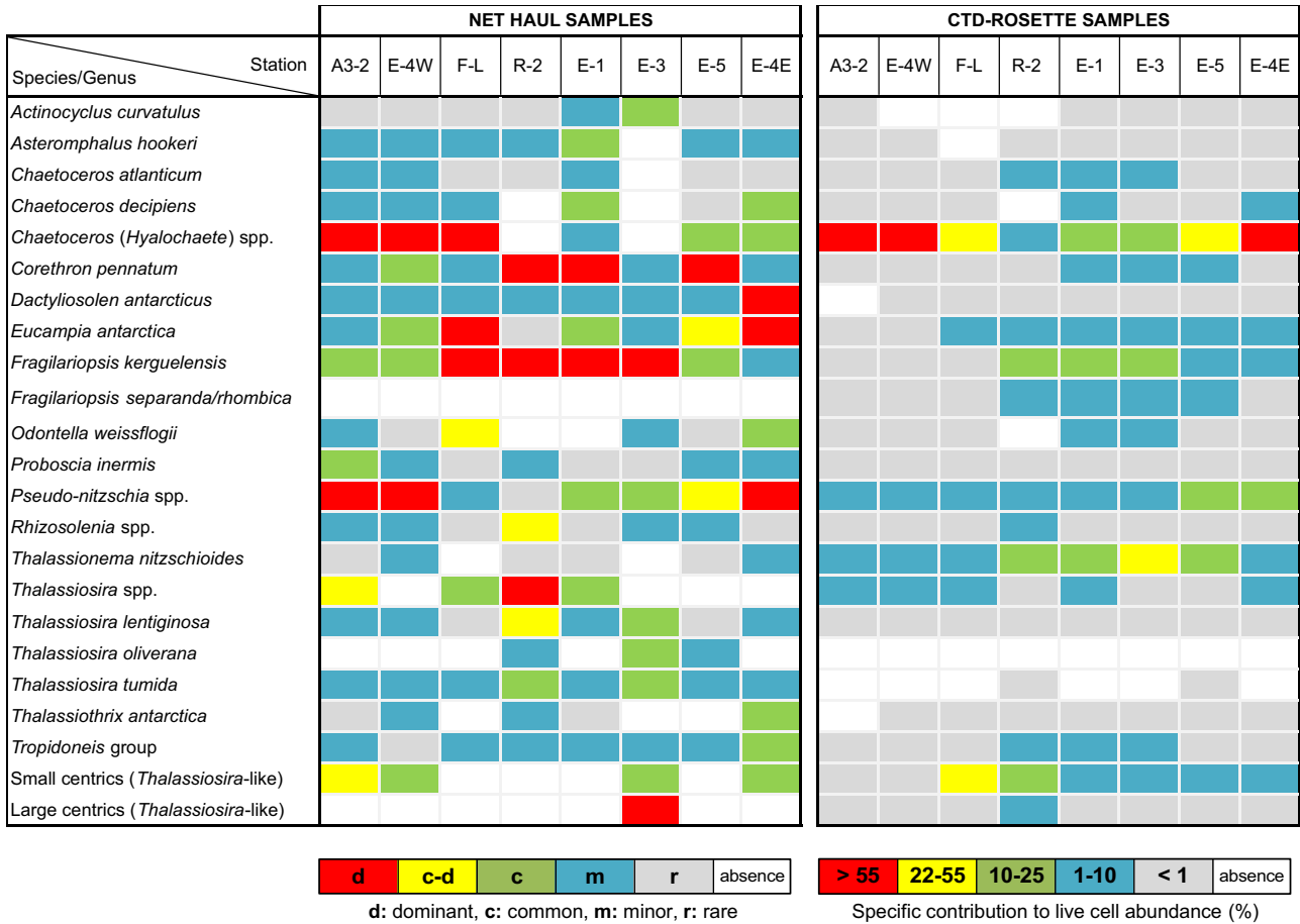
Figure 3. Qualitative assessment of diatom community composition from net hauls in the upper 100 m and comparison with the CTD rosette results averaged at all depths sampled over the water column. Only the main diatom species or genera observed over the study area are reported in this figure.
