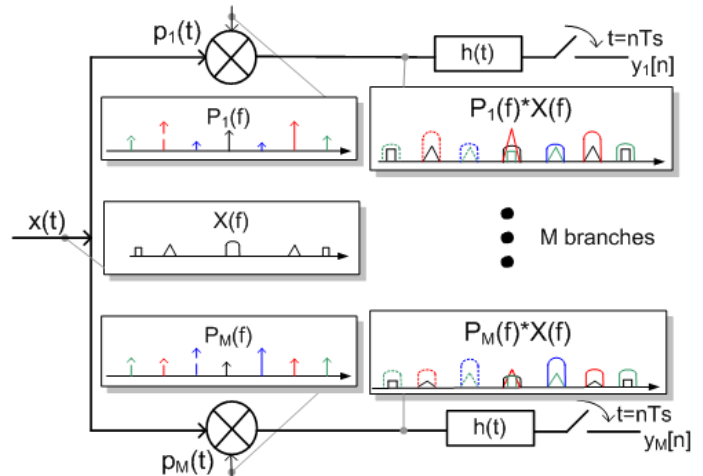
Fig. 1: Sensing process of the MWC.
