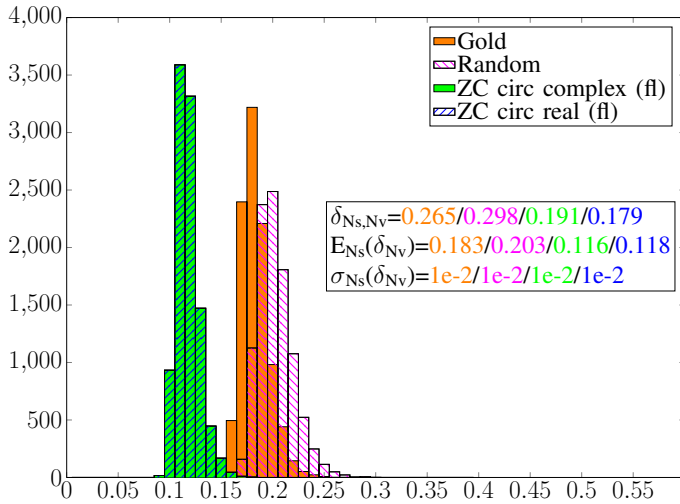
Fig. 3: Histogram of RIP-delta estimation (10000.10000).
