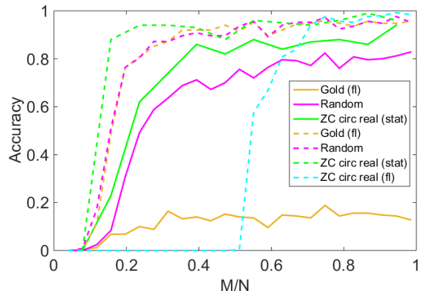
Fig. 5: Accuracy of the MWC with growing compression rate ( K=6 , 200 trials, OMP reconstruction algorithm), solid:10 dB ISNR, dashed: noiseless.
