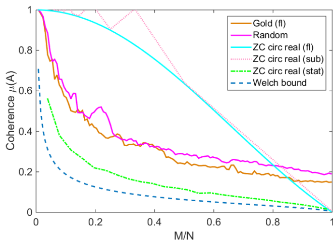
Fig. 2: Coherence comparison ( N=255 , R=1 ).
