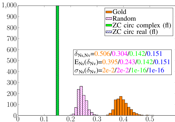
Fig. 4: Histogram of JLL-delta estimation (1000.1000).
