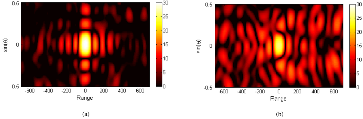
Fig. 1. Target amplitude estimation based on matched filter for one point target
