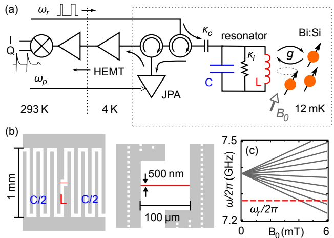
FIG. 1. (a) Schematic of the experiment: Bi:Si spins, biased by a dc magnetic field B_0 , are coupled to a LC resonator of frequency \omega_r . Microwave control pulses at \omega_r are sent onto the resonator input. The reflected signal, as well as the signals emitted by the spins, are first amplified by a JPA operated in degenerate mode followed by further amplification and homodyne demodulation to obtain the signal quadratures I(t) and Q(t) . (b) Design of the planar lumped element LC resonator. (c) ESR-allowed transitions of the Bi donor spins vs. B_0 . Dashed line indicates the resonator frequency.
