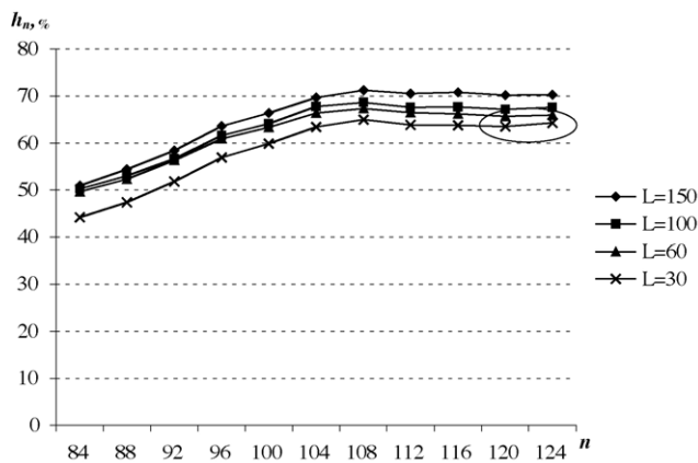
Fig. 8. Homogeneity ratios calculated for different rectangular area number L , showing the effect of the small structural default (circle line).
