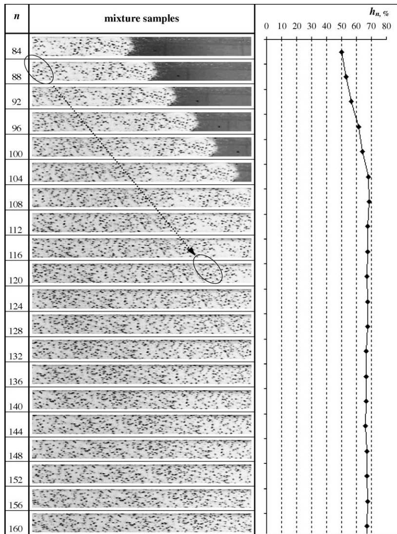
Fig. 7. Mixture samples and calculated homogeneity ratios ( L=100 ), showing a small structural default (circle line).
