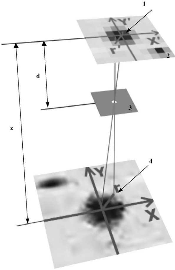
Fig. 2. Pinhole camera model (1, image coordinates; 2, image plane; 3, pinhole camera; 4, world coordinates).
