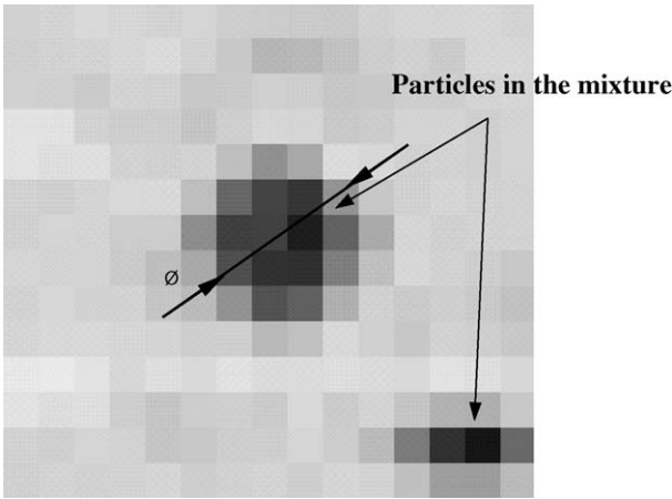
Fig. 3. Example of sampled and quantized binary mixture image.
