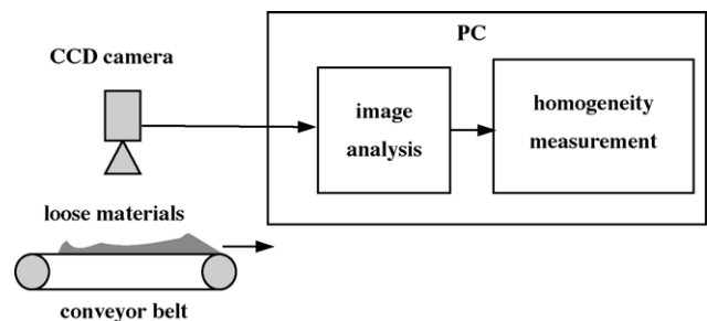
Fig. 1. Schematic diagram of the solid mixture analysing set-up.
