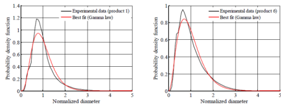
FIG. 3. The estimated probability density function of fiber diameter is shown for products 1 (left panel) and 6 (right panel). Here, the diameter is normalized by its mean value (for confidentiality reasons).
