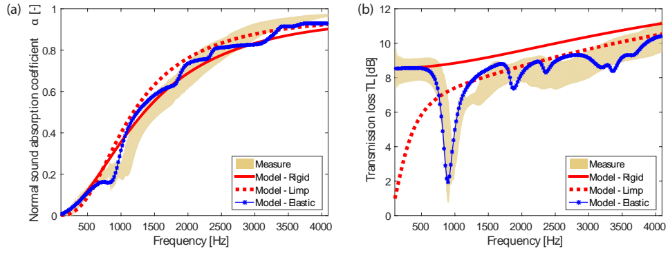
Figure 5: Comparison between measurements and prediction: (a) normal incidence sound absorption coefficient, (b) transmission loss. The sample thickness is equal to 14.30 \pm 0.89mm .
