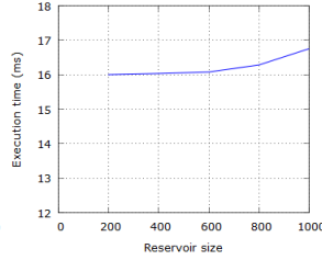
Fig. 5: Reservoir.
