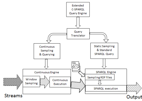
Fig. 3: C-SPARQL extended architecture
