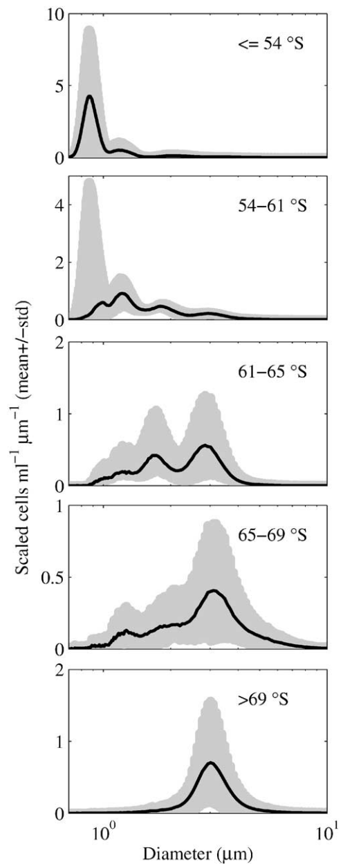
Fig. 9. Mean and standard deviation of the size distribution of phytoplankton in the upper 40 m for latitudinal bands on the Polar Front transect. Observations for the southbound and northbound transects were pooled. As in Fig. 8, each observed size spectrum was scaled to the same concentration of cells to provide an indication of changes in shape irrespective of changes in phytoplankton abundance.
