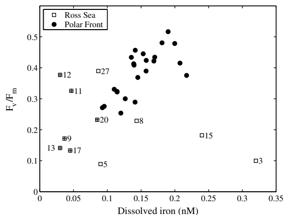
Fig. 13. Relationships between F_v/F_m and dissolved Fe concentration for both cruises. All values are the mean of observations in the upper 40 m of the water column, except for iron in the Ross Sea, where 60 m was used (because there was often only one measurement in the top 40 m). F_v/F_m values were derived from all cells measured by PDP flow cytometry in the Ross Sea and from in situ FRR measurements on the Polar Front transect. Station numbers are noted to the right of data points for the Ross Sea (see Fig. 1), and stations with one or more iron value at or below the detection limit of 0.03 nM are also indicated (+). For the Polar Front transect, r^2 = 0.50 .
