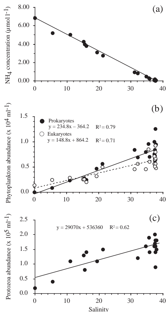
Fig. 3. (a) \text{NH}_4 concentration, (b) phytoplankton and (c) protozoa abundance versus salinity values. Line in (a) corresponds to theoretical values for \text{NH}_4 if only dilution process occurred; lines in (b) and (c) are regression lines obtained from linear regression models computed between abundance and salinity
