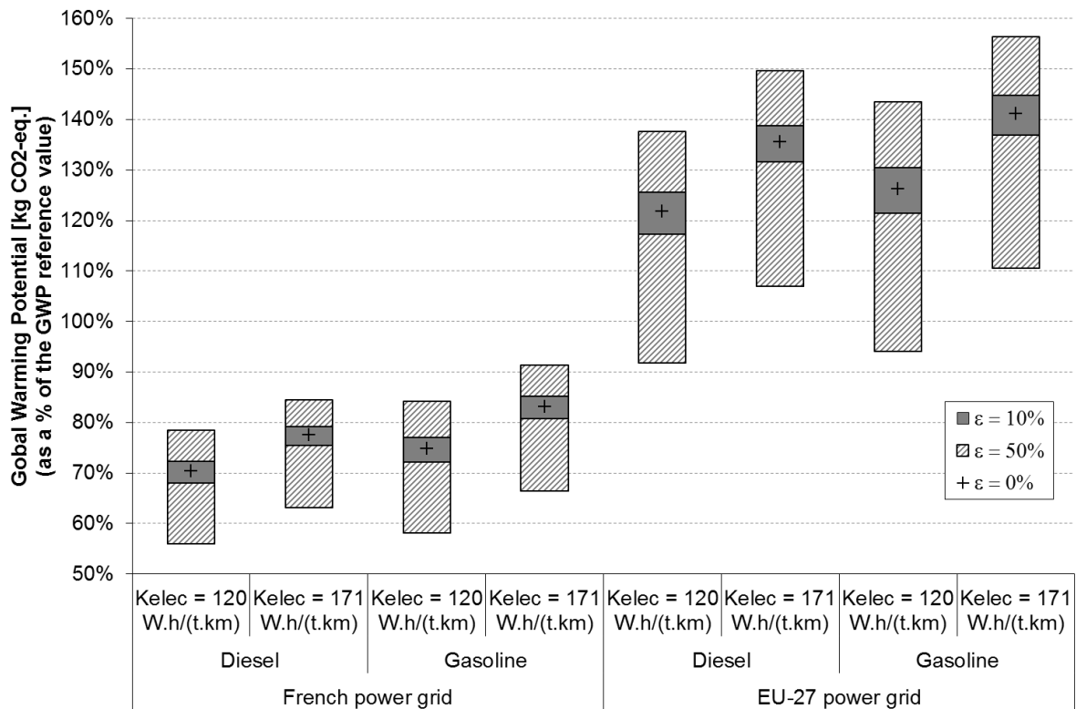
Figure 7. Sensitivity results of the GWP of the electricity mass consumption of the vehicle with and without air conditioning. For each value, three domain of variation are used. 100% reference is considered to be the life cycle GWP value of the input battery with French power grid and Diesel.
