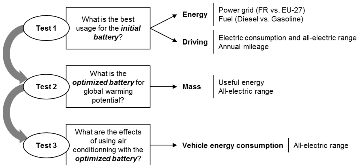
Figure 3. Schematic description of the experimentation with test goals and observed phenomena
