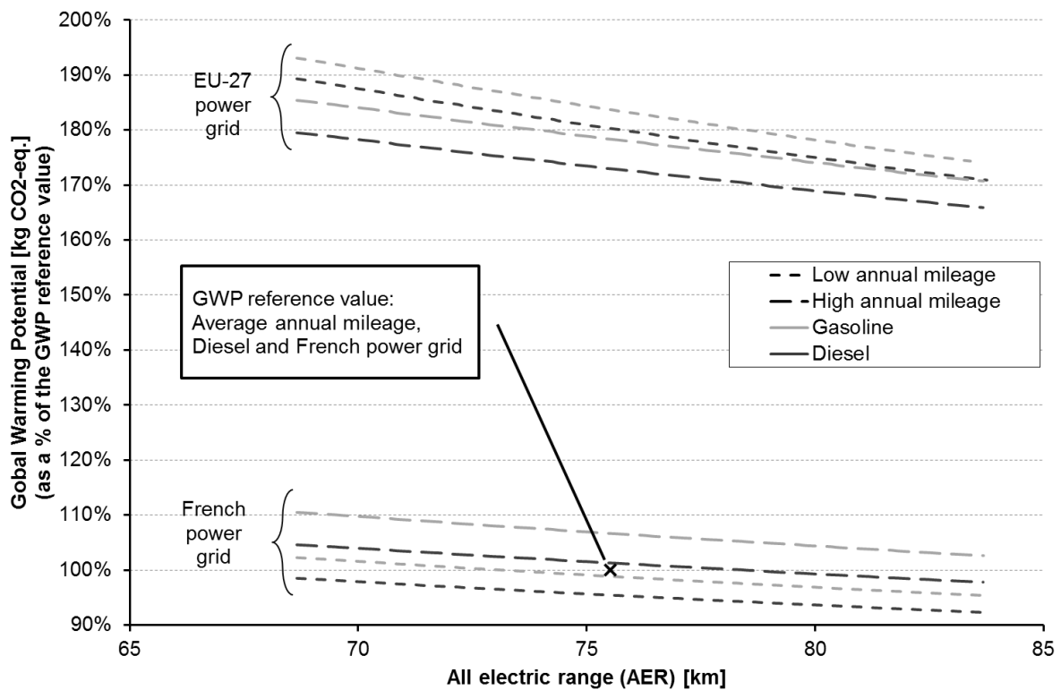
Figure 5. Evolution of the global warming potential as a function of the all-electric range, for EU-27 and French electricity mixes, gasoline and Diesel fossil fuels, and low and high annual mileages. 100% reference is considered to be the life cycle GWP value of the input battery with French power grid and Diesel.
