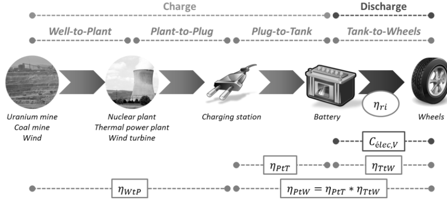
Figure 2. Electricity Well-to-Wheels cycle.
