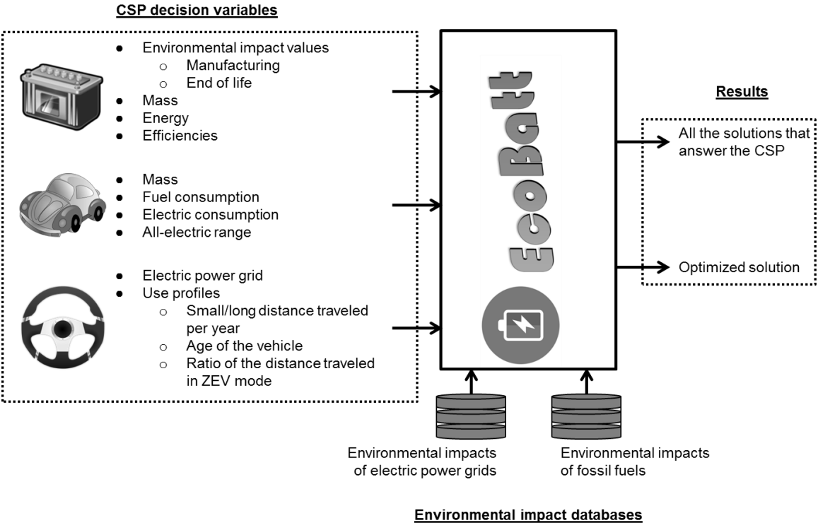
Figure 1. Schematic overview of EcoBatt inputs
