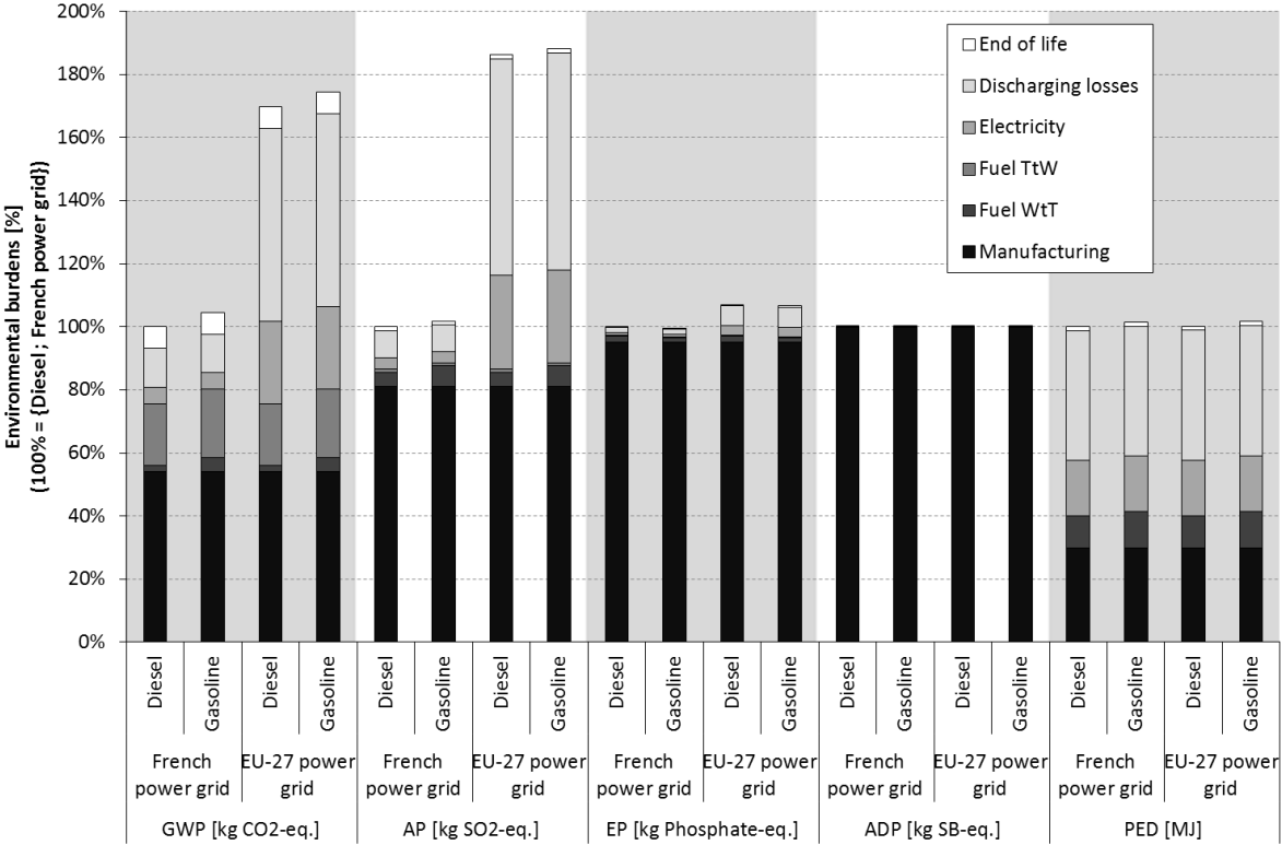
Figure 4. Environmental profile of the input Li-ion battery for a PHEV obtained from a LCA software. 100% reference is considered to be the life cycle impacts of Diesel PHEV on French power grid.
