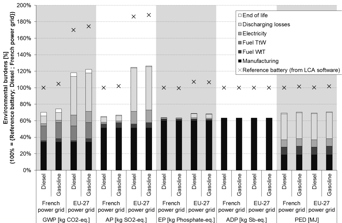
Figure 6. Environmental profile of the resized Li-ion battery. 100% reference is considered to be the life cycle impacts of the input battery with French power grid and Diesel.
