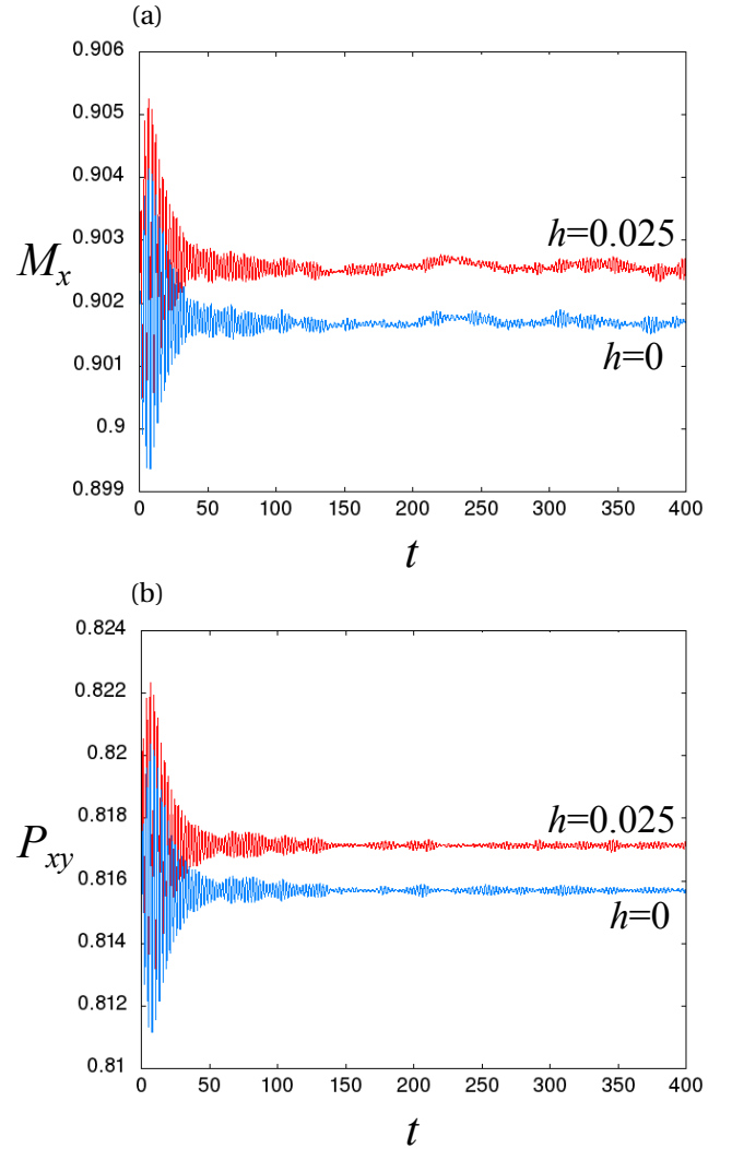
FIG. 2. (Color online) Time series of order parameters: The panel (a) is the time series for M_x and the panel (b) for P_{xy} . The temperature T = 0.3 , the number of particles N = 4 \times 10^6 , and the time step \delta t = 0.05 . For each panel, the upper (red) curve is for h = 0.025 and the lower (blue) one for h = 0 .
