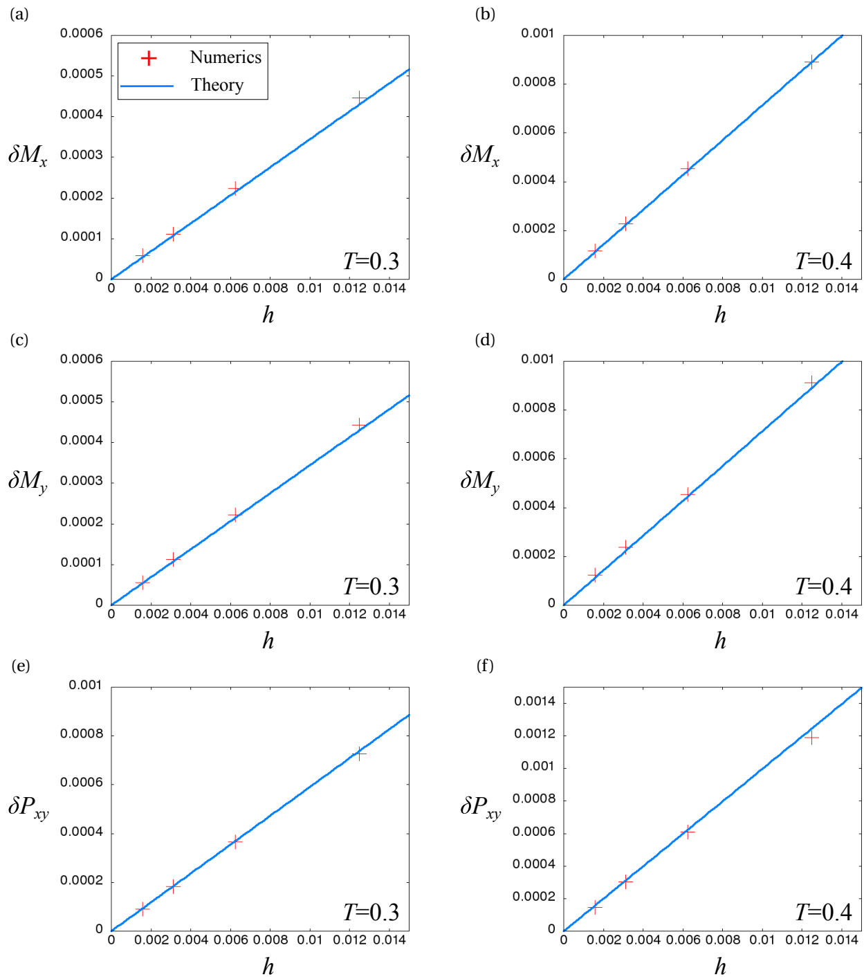
FIG. 3. (Color online) \delta M_x , \delta M_y , and \delta P_{xy} as functions of h . The lines are the linear responses obtained theoretically and the crosses are responses obtained numerically. We set temperature of the initial states as T = 0.3 (Left column, panels (a, c, e)) and T = 0.4 (Right column, panels (b, d, f)), and a number of particles N = 4 \times 10^6 and the time step \delta t = 0.05 .
