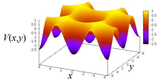
FIG. 1. (Color online) The effective potential of the Hamiltonian (41). A minimum point is at (0, 0) and \min \mathcal{V} = -2M - P . Saddle points are at (\pm\pi, 0) and (0, \pm\pi) and \mathcal{V} = P . A maximum point are on (\pm\pi, \pm\pi) and \max \mathcal{V} = 2M - P , where M > P > 0 .
