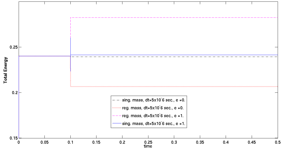
FIGURE 13. Energy evolution. Argyris element, 80 triangles. \Delta t = 5 \times 10^{-6} . e - \beta -Newmark scheme. e = 0 or e = 1 , regular or singular mass matrices.
