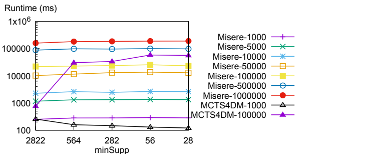
Fig. 22: Runtime of MISERE and MCTS4DM when varying minSupp on the Mushroom dataset.
