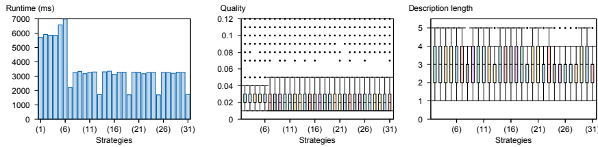
(a) Runtime: BreastCancer (b) Avg. quality: Mushroom (c) Descr length: Mushroom
