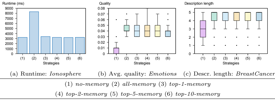
Fig. 9: Impact of the MEMORY strategy.
