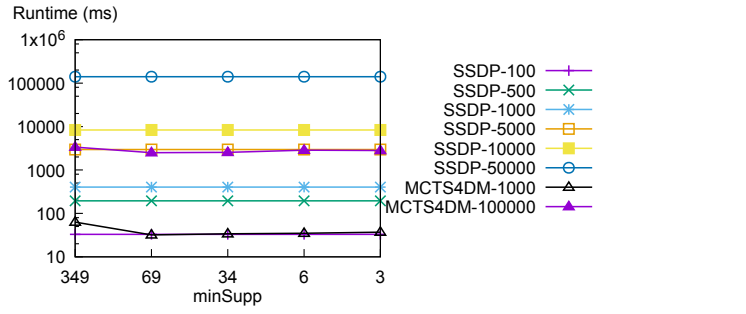
Fig. 19: Runtime of SSDP and MCTS4DM when varying minSupp in Breast-Cancer .
