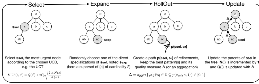
Fig. 4: A simple instantiation of MCTS for pattern mining.
