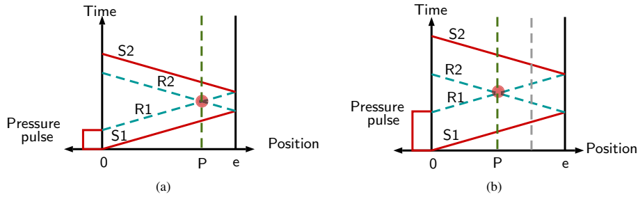
Fig. 2. Time/position diagrams in the case of one pulse laser shock – pressure pulse duration is longer in (b) than in (a).
