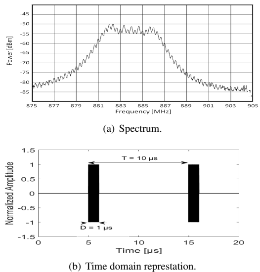
Figure 3. Spectrum and time domain representation of the interference applied.
