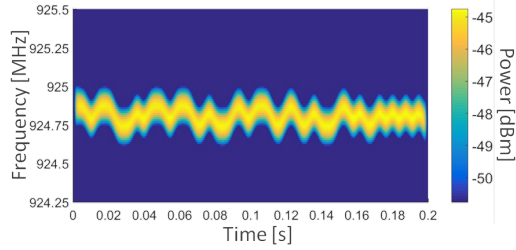
Figure 1. Time-frequency representation of a GSM-R signal.
