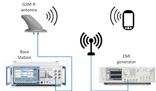
Figure 2. Diagram of the test bench used.
