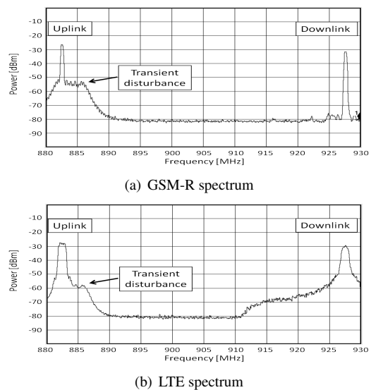
Figure 4. Spectra of used GSM-R and LTE networks in presence of repeated transient interferences.
