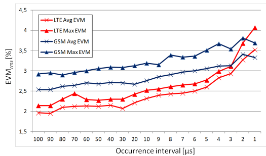
Figure 5. Average and maximum EVM_{rms} of GSM-R and LTE communications for different interval of occurrence of the transient disturbance.
