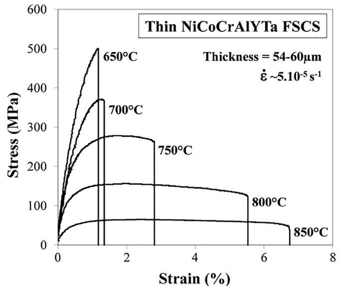
Fig. 6. Stress-strain curves of the thin NiCoCrAlYTa Tribomet® FSCS between 650 °C and 850 °C.
