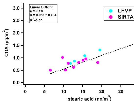
Fig. 7. Comparison of stearic acid (GC-MS) and COA (PMF) concentrations.
