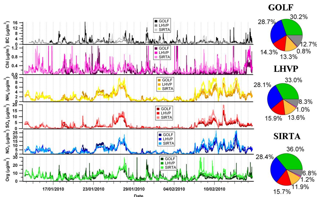
Fig. 1. Comparison of PM 1 chemical composition from AMS (organics (Org), sulfates (SO 4 2- ), nitrates (NO 3 - ), ammonium (NH 4 + ), chlorine (Chl)) and black carbon (BC) measurements in the Paris region.
