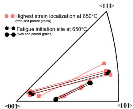
Fig. 20 An IPF map with superimposed parent-twin grain pair orientations connected via lines. In red , the orientations of the grain pairs exhibiting the highest strain localization as measured using SEM DIC in LCF. In black , the orientations of grain pairs measured from LCF initiated cracks that led to failure when tested at 650 °C
