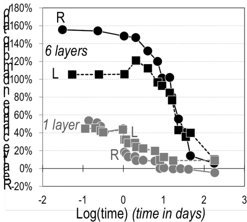
Figure 1: Changes trough time (7months) of vibration damping of mulberry wood varnished with Sandarac dissolved in ethanol. 1 data point = mean of 6 specimens, Time axis in Log-scale (0=1day, 1=10days, 2=100days).
