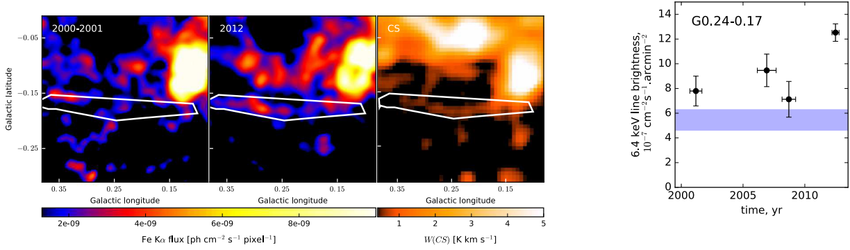
Fig. 14. Left images: Fe K\alpha maps centred at the position of the G0.24–0.17 filament during the 2000–2001 and 2012 XMM-Newton observations. The maps are in units of \text{ph cm}^{-2} \text{s}^{-1} \text{pixel}^{-1} , with 2.5'' pixel size, and smoothed using a Gaussian kernel of 8 pixels in radius. Centre: Mopra CS(1–0) map integrated over the 27–35 \text{km s}^{-1} velocity band. Right: Fe K\alpha light curve of the G0.24–0.17 filament. The blue band indicates the level of background emission measured in a circular region south of Sgr A*. All errors shown on the light curves are 1\sigma errors (68% confidence level).
