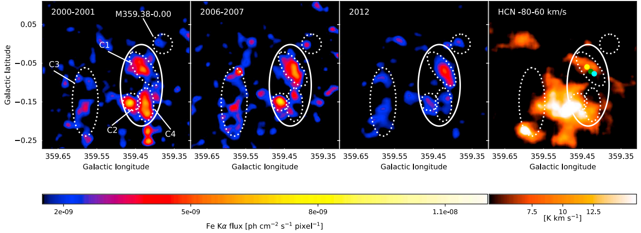
Fig. 10. Fe K\alpha maps of the Sgr C complex for three periods of XMM-Newton observations ( first three panels from the left ) and Mopra HCN map integrated over the -80 to -60 km s^{-1} velocity band for the same region ( right panel ). The yellow, green, and cyan dots give the position of the centroid of the emission in the C1 region in 2000–2001, 2006–2007 and 2012, respectively. A displacement of 1.6' of the emission in a direction similar to that of the molecular feature is visible. The Fe K\alpha maps are in units of \text{ph cm}^{-2} \text{s}^{-1} \text{pixel}^{-1} , with 2.5'' pixel size, and smoothed using a Gaussian kernel of 8 pixels radius. The solid line region labelled Sgr C includes the bulk of the Fe K\alpha bright clumps, while the smaller regions reported by other papers plus the C4 clump newly labelled here are shown in dotted lines.
