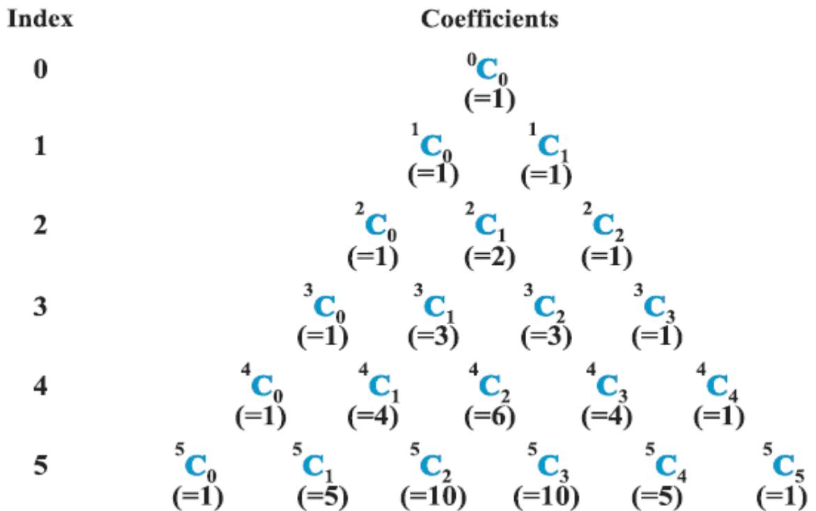
Figure 4. Pascal's Triangle
