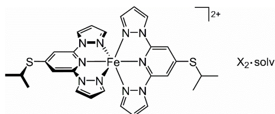
Scheme 1. Compound 1 X_2 \cdot \text{solv} ( X^- = \text{BF}_4^- or \text{ClO}_4^- ; solv = \text{MeNO}_2 , \text{MeCN} , \text{Me}_2\text{CO} , \text{H}_2\text{O} or sf [solvent-free]).
