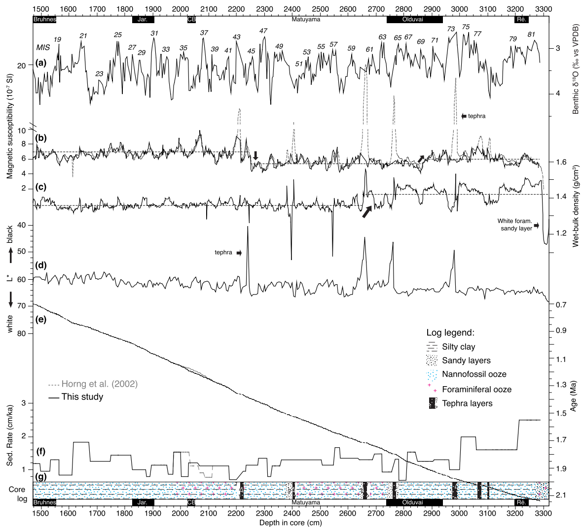
Fig. 2. Chronology and sedimentological description of core MD97-2143. (a) Benthic \delta^{18}\text{O} ( Cibicides wuellerstorfi ) record (Horng et al., 2002) and marine isotopic stages (MIS). (b) Magnetic susceptibility measured on individual samples (black line) and on the whole core (grey dashed line). (c) Wet-bulk density and (d) sediment lightness ( L^* ). (e) The original ages model of Horng et al. (2002) and its derived sedimentation rates (f) have been slightly adjusted around the MIS 35/36 transition in this study (see text and supplementary Fig. S1). (g) Sediments description is synthesis in a core log based on the IPHIS mission report and physical data.
