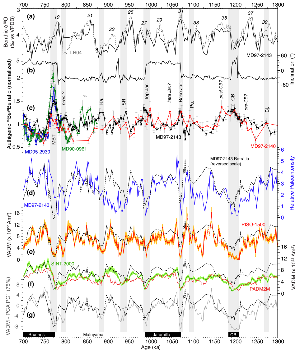
Fig. 7. Geomagnetic field changes in the 700–1300 ka time interval. (a) Benthic \delta^{18}\text{O} record in black compared to the LR04 stack in grey. (b) MD97-2143 inclination. (c) Normalized Be-ratios of MD97-2143 (black), MD05-2930 (blue; Ménabréaz et al., 2014), MD90-0961 (green; Valet et al., 2014), MD97-2140 (red; Carcaillet et al., 2003). (d) MD97-2143 RPI record. (e–f) RPI stacks: (e) PISO-1500 (Channell et al., 2009), (f) SINT-2000 (green, Valet et al., 2005) and PADM2M (red, Ziegler et al., 2011). (g) The first principal component extracts by PCA analysis on the PISO-1500, SINT-2000 and PADM2M records (grey curve) explains 75% of the variance and yields a series of GDL in phase with ^{10}\text{Be} overproduction episodes. (d–g) The MD97-2143 Be-ratio (black dashed line) is plotted on a reversed scale. Geomagnetic events (reversals and excursions) have been labeled and refer to the geomagnetic polarity time scale (bottom): MBT (Matuyama–Brunhes transition), Ka. (Kamikatsura), SR (Santa Rosa), Jar. (Jaramillo), Pu. (Punaru), CB (Cobb Mnt), Bj. (Bjorn Exc.). (For interpretation of the references to color in this figure legend, the reader is referred to the web version of this article.)
