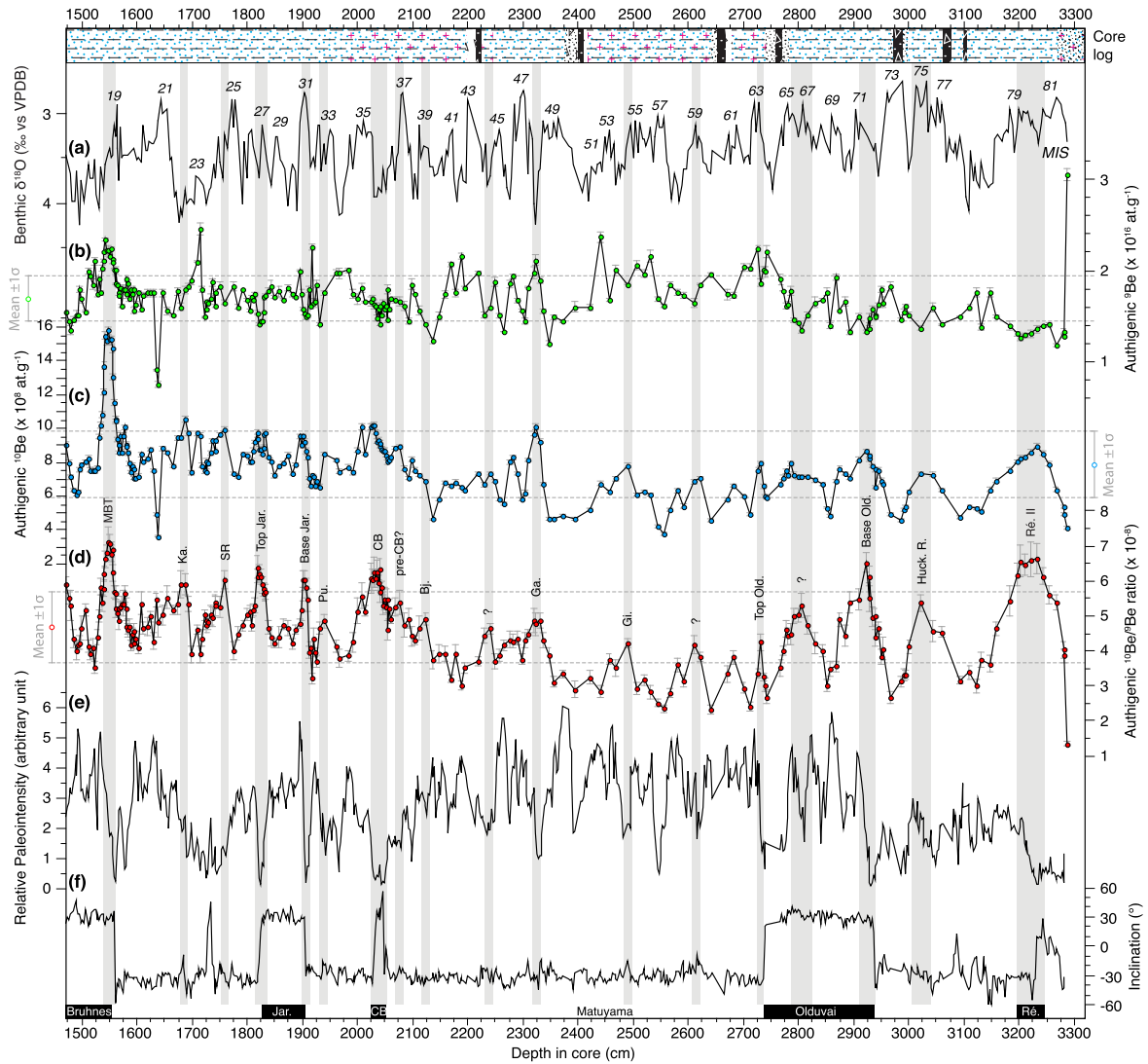
Fig. 3. Paleomagnetic and Be results of core MD97-2143. (a) Benthic \delta^{18}\text{O} record. (b) Authigenic ^9\text{Be} concentration. (c) Authigenic ^{10}\text{Be} concentration. (d) Authigenic ^{10}\text{Be}/^9\text{Be} ratio (Be-ratio). (e) Relative paleointensity (RPI) and (f) inclination. Geomagnetic events (reversals and excursions) have been labeled and refer to the geomagnetic polarity time scale (bottom): MBT (Matuyama–Brunhes transition), Ka. (Kamikatsura), SR (Santa Rosa), Jar. (Jaramillo), Pu. (Punaru), CB (Cobb Mnt), Bj. (Bjorn Exc.), Ga. (Gardar Drift), Gi. (Gilsa), Old. (Olduvai), Huck. R. (Huckelbury Ridge), Ré. (Réunion).
