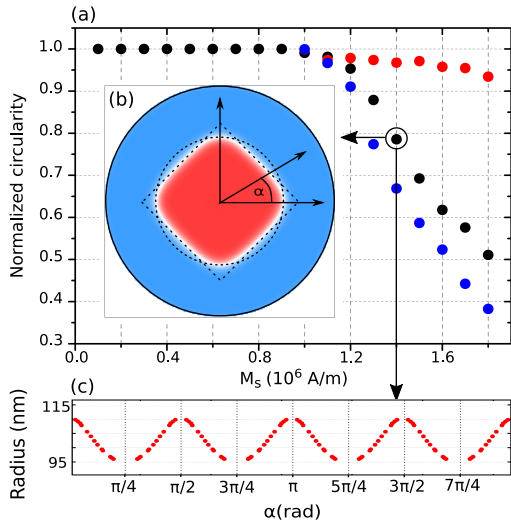
Figure 6: (a) Normalized circularity factor C_n as a function of M_s for an anti-skyrmion stabilized in dots with a diameter of 500 nm (blue), 400 nm (black) and 200 nm (red). (b) Magnetic configuration of an anti-skyrmion ( M_s = 1.4 \cdot 10^6 A/m, A_{\text{ex}} = 16 pJ/m, K_{\text{eff}} = 2 \cdot 10^5 J/m 3 , D = 2.0 mJ/m 2 ) with a sketch that shows the square-circular shape. (c) Radius of an anti-skyrmion as a function of the in-plane angle \alpha
