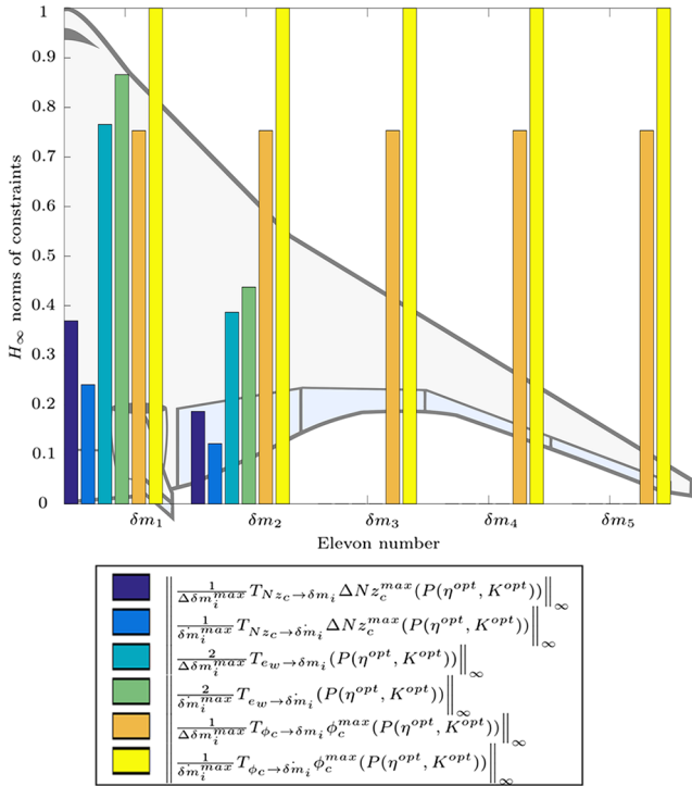
Fig. 11 Bar diagram of normalized constraint values after optimization with tunable allocation: \eta^{\text{opt}} = 0.3885 .
