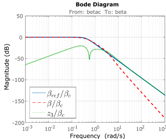
c) Comparison of directional reference model, closed-loop, and error frequency responses
