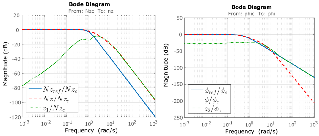
a) Comparison of longitudinal reference model, closed-loop, and error frequency responses
