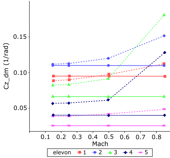
a) Comparison of lift gradient coefficients for reference aircraft: C_{L\delta m_i}^{ref} (dotted) vs C_{L\delta m_i}^{AVL} (plain)
