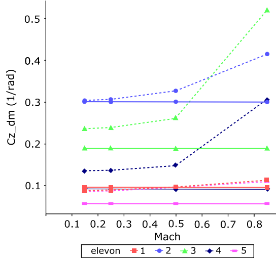
b) Comparison of lift gradient coefficients for project aircraft before (plain) and after calibration (dotted), respectively
