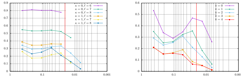
Figure 2. Energy-error as a function of the coarse-scale meshsize for various resolutions of the oscillatory basis functions (left) and for various values of k . The vertical red line indicates the value of \varepsilon .
