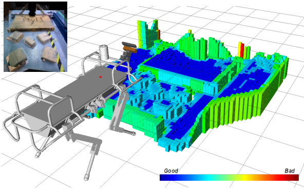
Fig. 2. The reward map generation from RGBD (Asus Xtion) camera data. The RGBD sensor is mounted on a PTU unit that scans the terrain. An occupancy map is built with a 2 cm resolution. Then the set of features is computed and the total reward value per pixel of 4 cm is calculated. In addition, a height map of 2 cm resolution in z is created. The reward values are represented using a color scale, where blue is the maximum reward and red is the minimum one.
