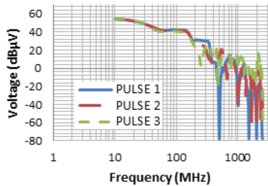
Fig 3. Comparison between the simulations using the different shapes of IA with a 1 \Omega probe
