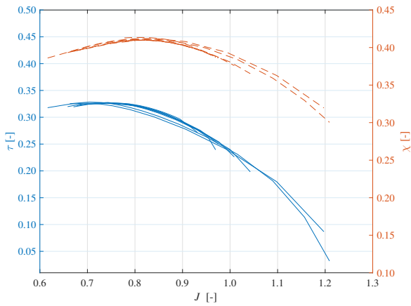
Figure 7 DGEN-380 (\tau, J, \chi) map
