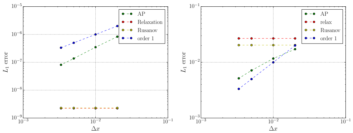
Figure 14: Density error (left) and velocity magnitude error (right) in terms of \Delta x for M = 0.1 (Travelling vortex).
